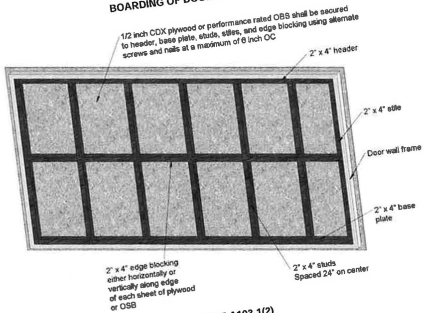
FIGURE A103.1(2) BOARDING OF DOOR WALL
