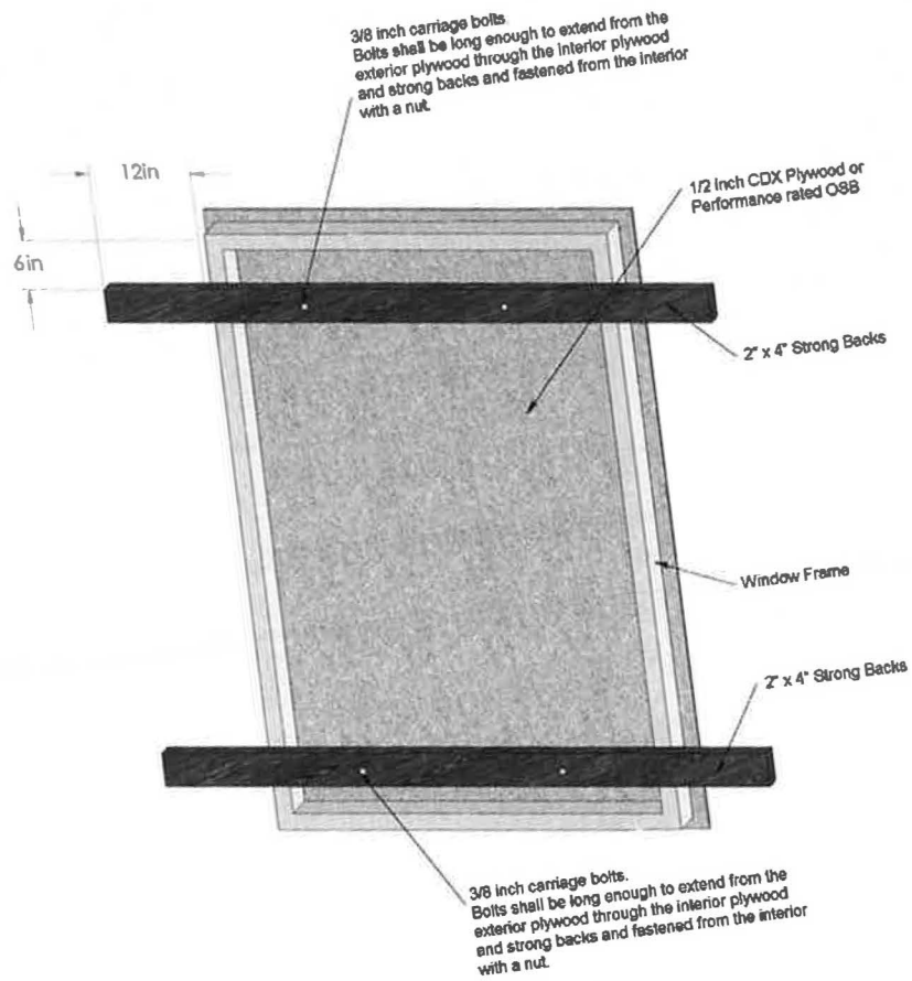
FIGURE A103.1(1) BOARDING OF DOOR OR WINDOW
